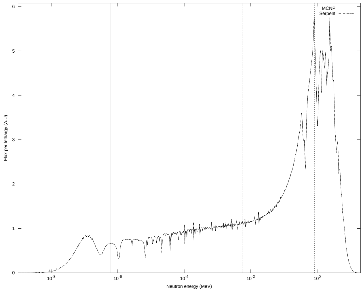
Figure 15. Flux spectra integrated over the entire geometry Mixed PWR MOX/UX lattice.
